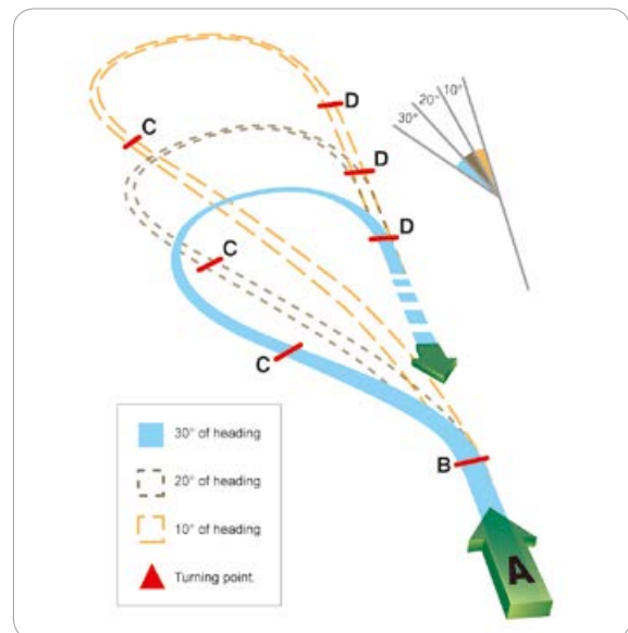
[그림 4-44] Teardrop pattern (entire pattern in level flight)
