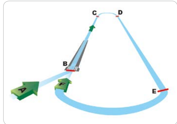
[그림 4-46] Patterns applicable to circling approaches II (runways are imaginary)
