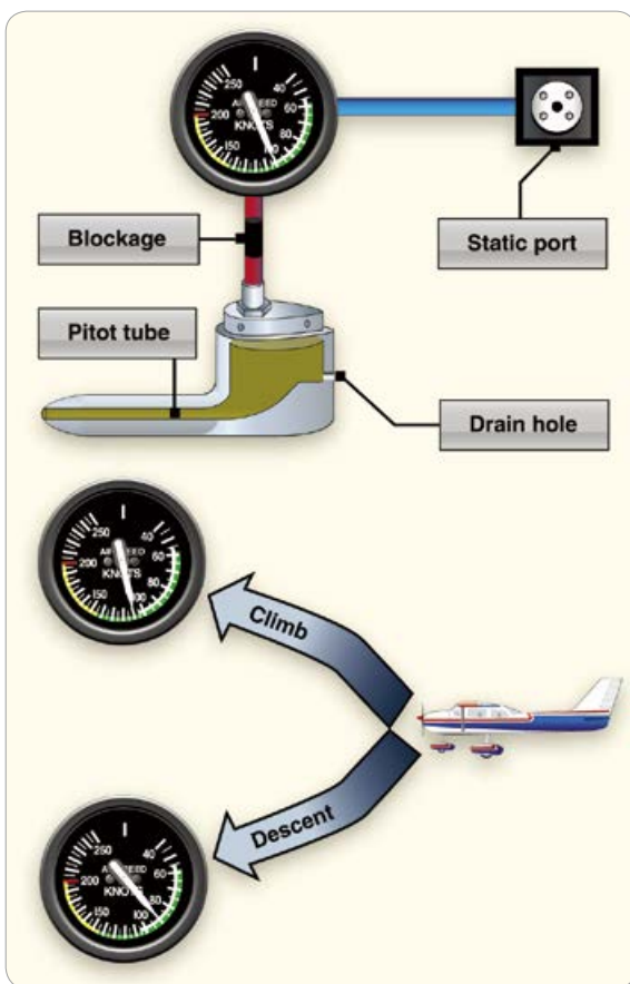
[그림 3-16] Blocked pitot system with clear static system
