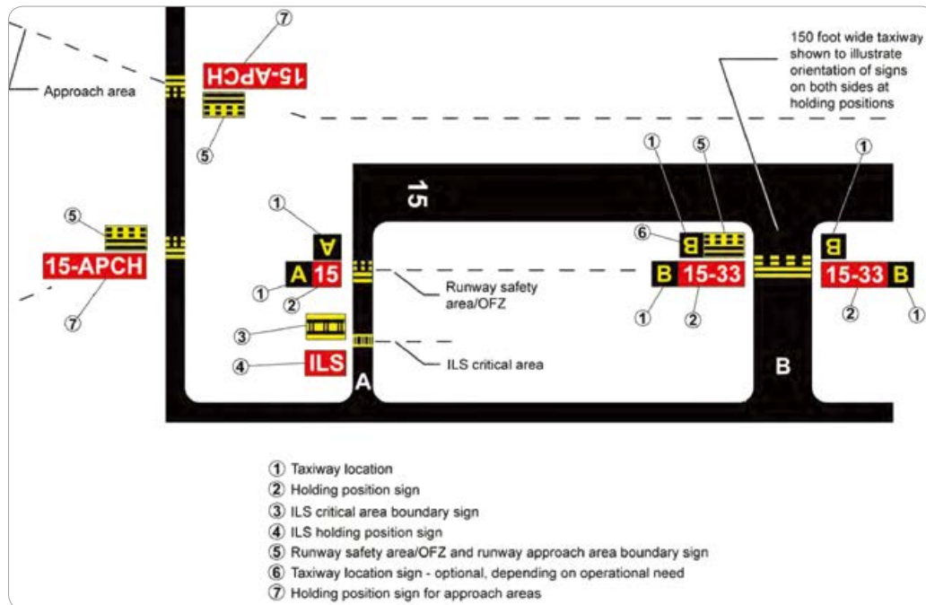
[그림 1-27] Taxiways Located in Runway Approach Area
