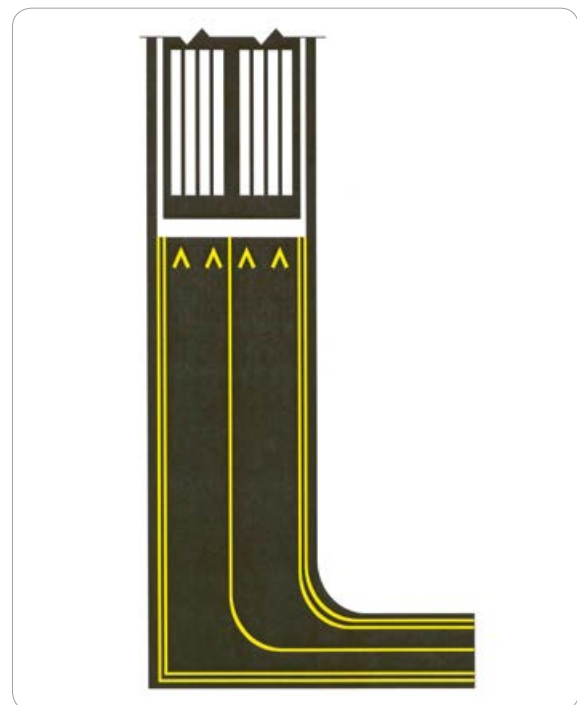
[그림 1-16] Relocation of a Threshold with Markings for Taxiway Aligned with Runway
