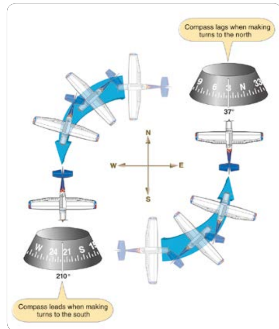
[그림 4-35] Northerly and southerly turn error
