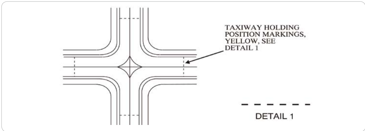
[그림 1-29] Holding Position Markings: Taxiway/Taxiway Intersections
