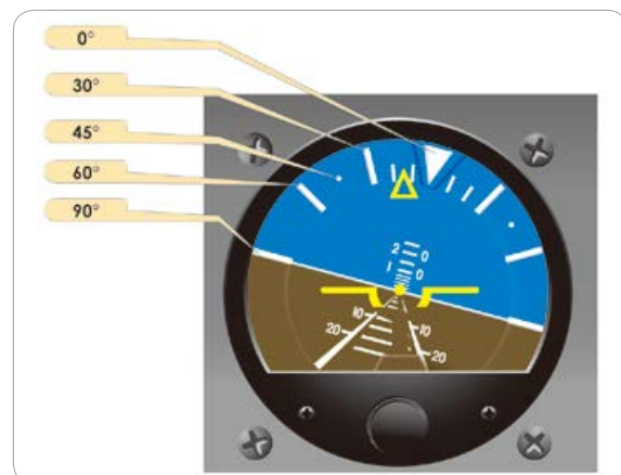
[그림 4-17] Bank interpretation with the attitude indicator
