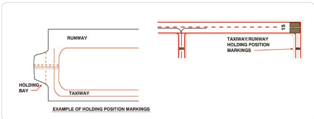
[그림 1-25] Runway Holding Position Markings on Taxiway
