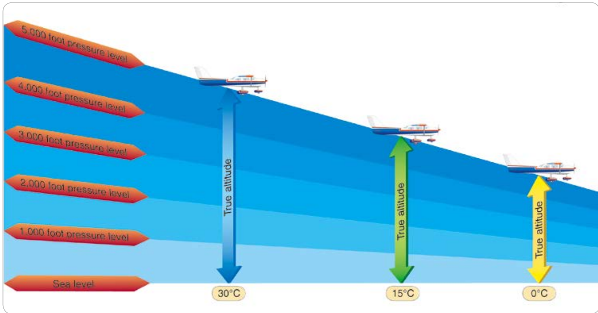
[그림 3-6] Effects of nonstandard temperature on an altimeter
