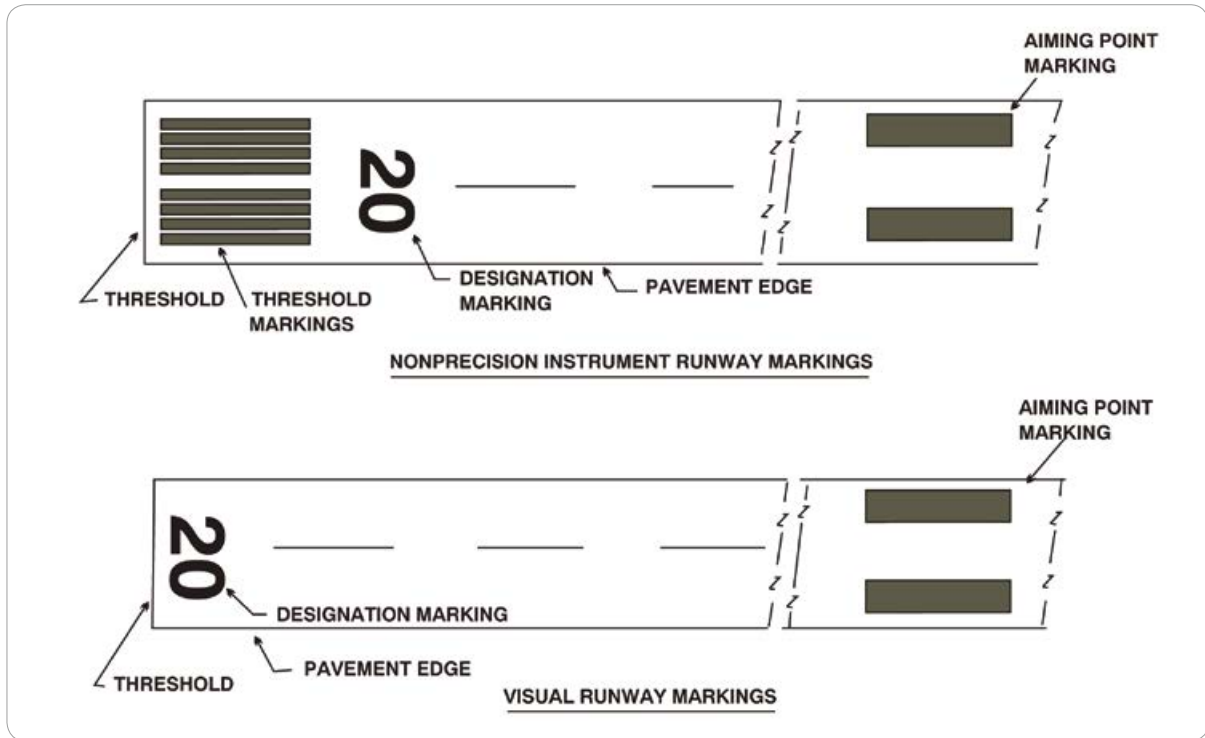
[그림 1-14] Nonprecision Instrument Runway and Visual Runway Markings
