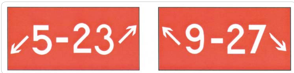
[그림 1-33] Holding Position Sign for a Taxiway that Intersects the Intersection of Two Runways
