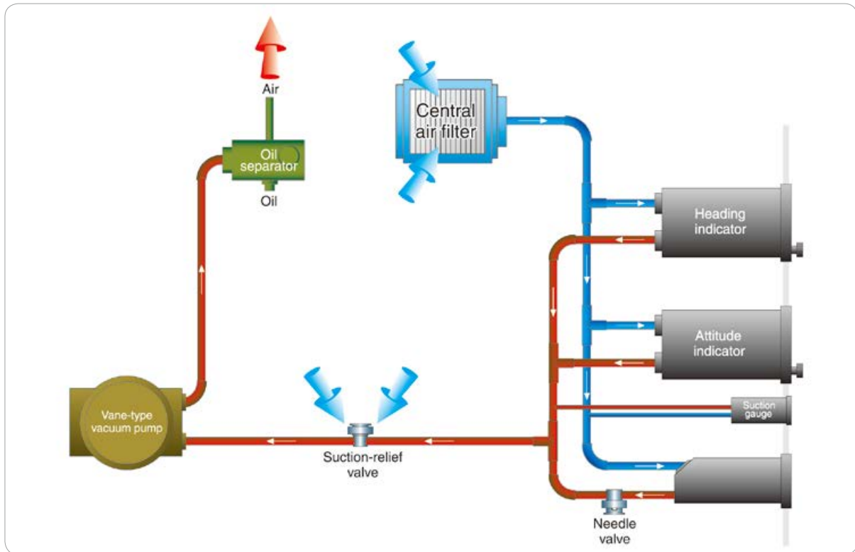
[그림 3-25] Single-engine instrument vacuum system using a steel-vane wet-type vacuum pump
