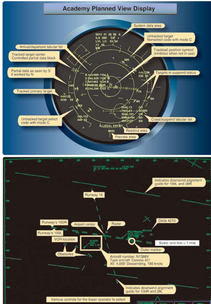
[그림 8-6] The top image is a display as seen by controllers in an air traffic facility
