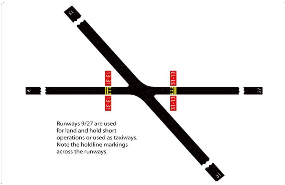
[그림 1-26] Runway Holding Position Markings on Runways
