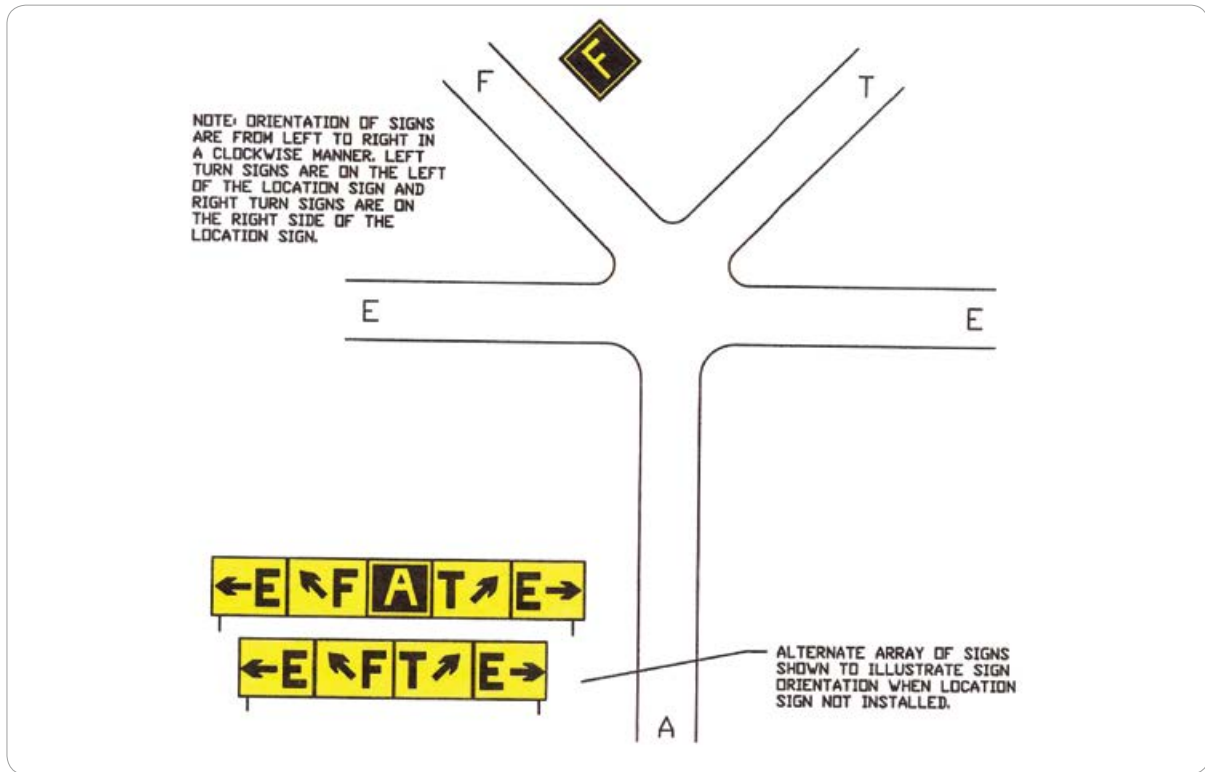
[그림 1-42] Direction Sign Array with Location Sign on Far Side of Intersection
