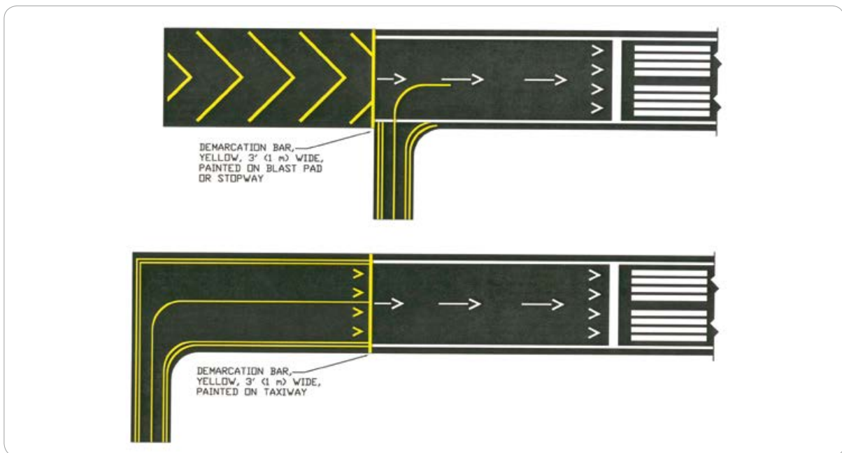
[그림 1-19] Markings for Blast Pad or Stopway or Taxiway Preceding a Displaced Threshold
