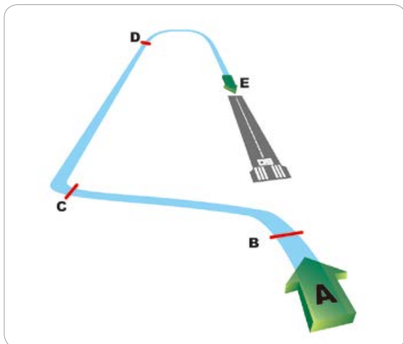
[그림 4-45] Patterns applicable to circling approaches I (runways are imaginary)
