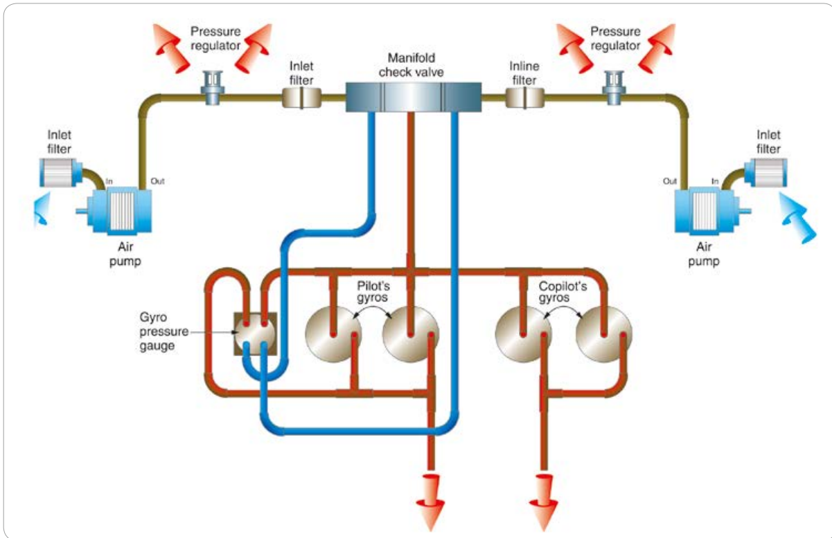
[그림 3-26] Twin-engine instrument pressure system using a carbon-vane dry-type air pump
