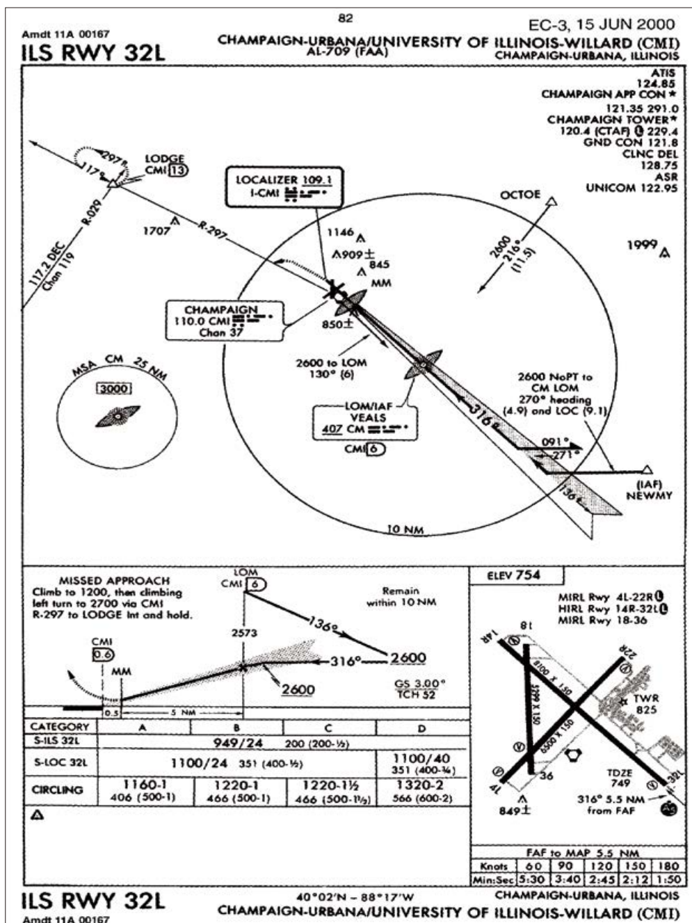
[그림 5-11] Champaign, IL(CMI) ILS Rwy32L approach
