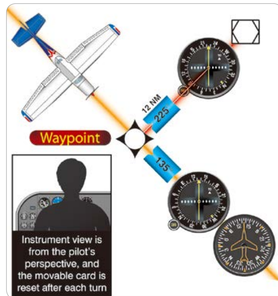
[그림 2-24] Aircraft/VORTAC/waypoint relationship
